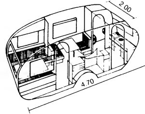
10 Caravan with areas for cooking and eating
